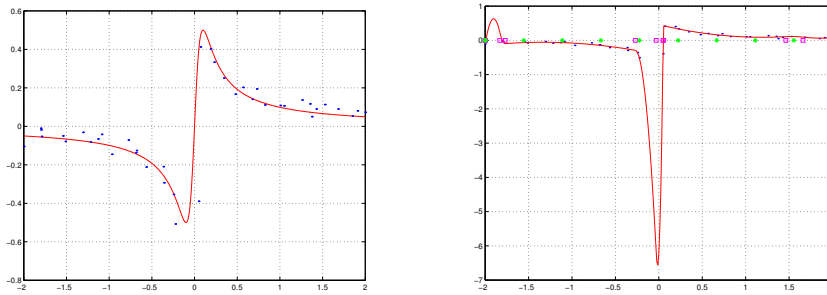
Figure 2. Example 1: The function 10x/(1+100x^2) and noisy data (left) and raw approximation with 11 quadratic B-splines (right; \varepsilon = 0.001 )
