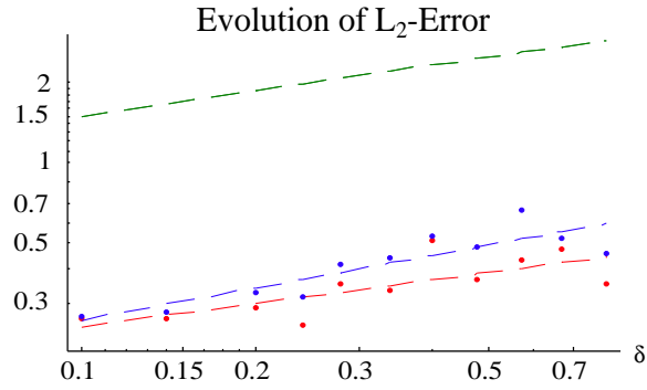
Figure 8: Evolution of the L_2 -norm of the difference f^\delta - f_k^\delta (blue) and f - f_k^\delta (red) for noise level tending to zero. The green line indicates the rate which is obtained for the stopping rule.
