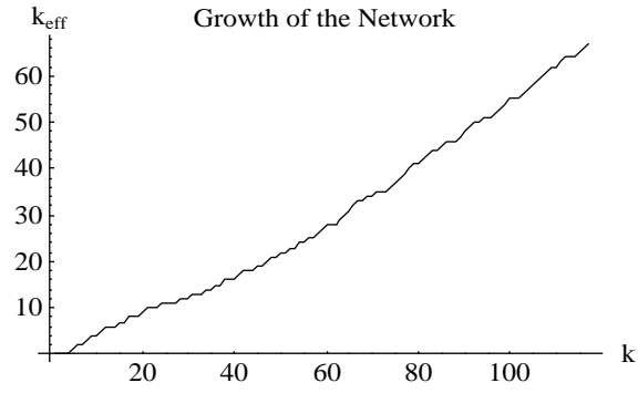
Figure 3: Evolution of the network size during the greedy algorithm.
