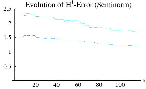
Figure 5: Evolution of the H^1 -seminorm of the difference f - f_k . The upper line corresponds to \|\partial_{x_1}(f - f_k)\|_{L_2(\Omega)} , the lower one to \|\partial_{x_2}(f - f_k)\|_{L_2(\Omega)} .
