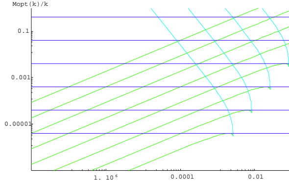
Figure 10: Behaviour of \frac{M(k_i)}{k_i} corresponding to the three different choices for k in Section 3.3. The lower curves correspond to the choice \gamma = 10^{-6} , the top ones to \gamma = 10^{-1} .
