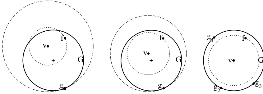
Figure 1: Interpretation of condition (2.1). The objective function is the difference of the radii of the two dashed circles. In this symmetric case the infimum is attained for v lying in the center of G .
