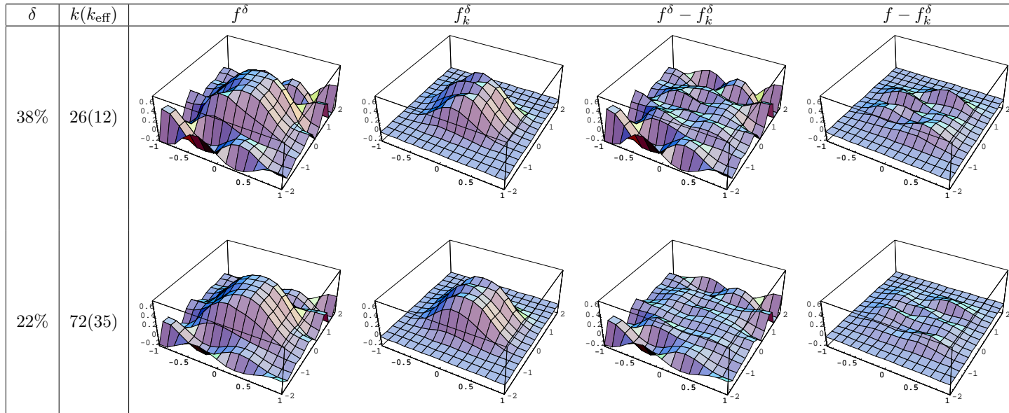
Figure 12: Behaviour of the algorithm for noisy data and two different noise levels.
