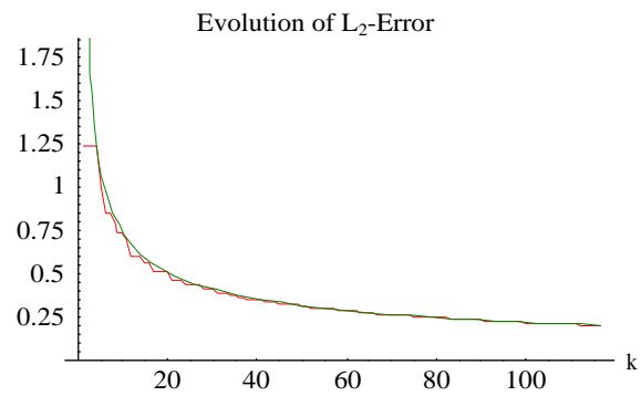
Figure 4: Evolution of the L_2 -norm of the error f - f_k .
