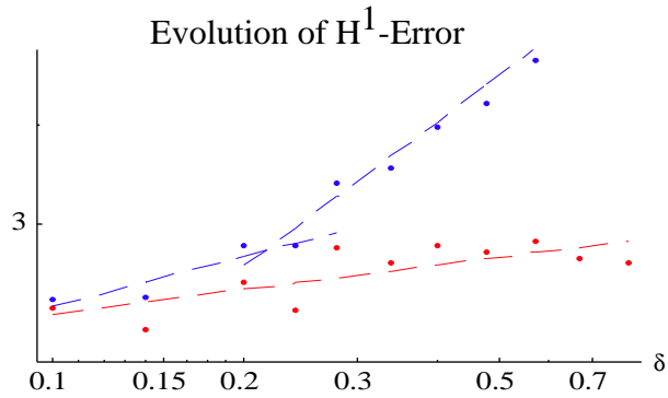
Figure 9: Evolution of the H^1 -norm of the difference f^\delta - f_k^\delta (blue) and f - f_k^\delta (red) for noise level tending to zero.
