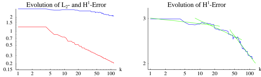
Figure 6: Logarithmic plot of the evolution of the L_2 -norm (red) and the H^1 -norm (blue) of the difference f - f_k . The right graph is a magnification of the left one and shows interpolations of the H^1 -error (green). The slope is gradually increasing.
