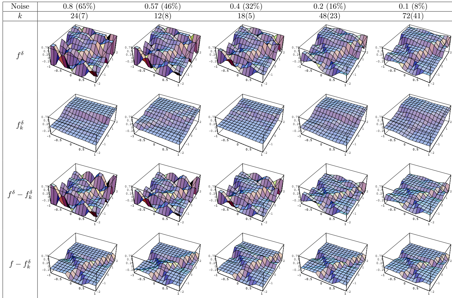
Figure 7: Qualitative behaviour of the algorithm for noise level tending to zero.
