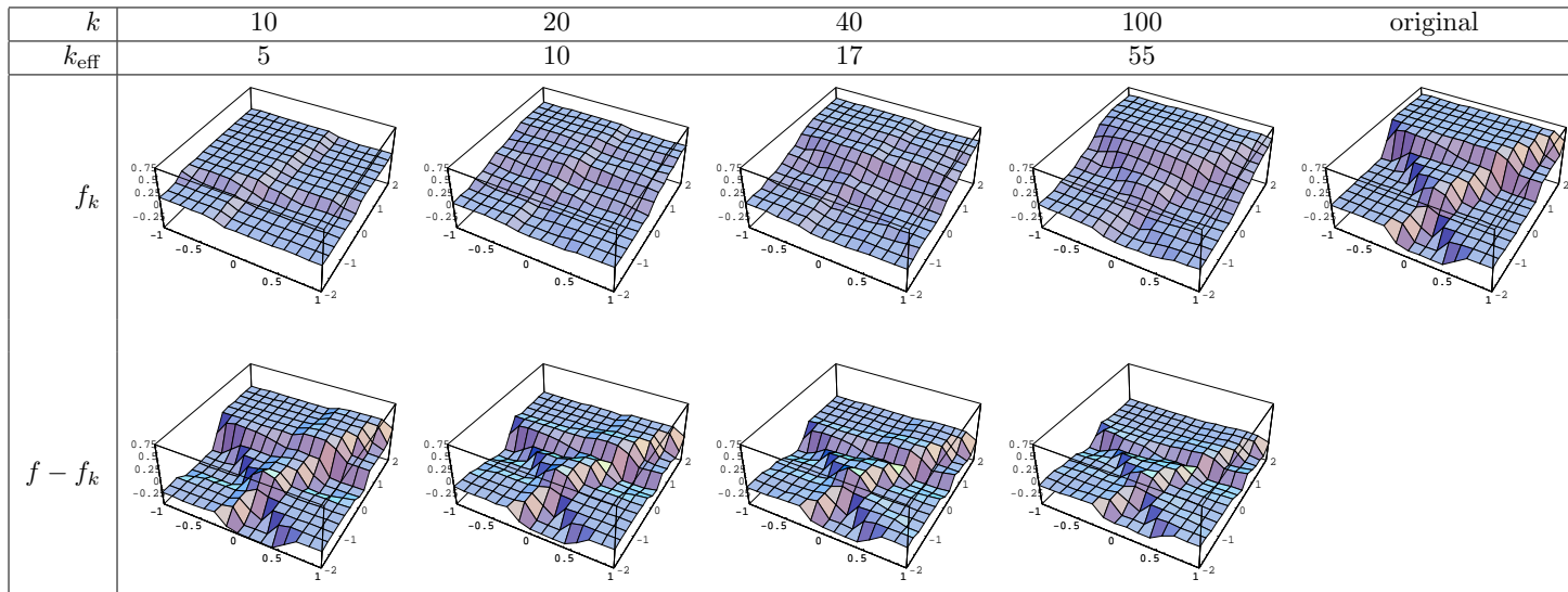
Figure 2: Evolution of the approximation f_k and the error f_k - f during the greedy algorithm.
