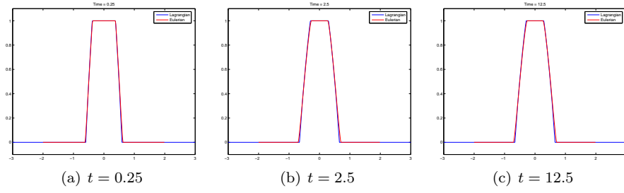
FIGURE 3. Comparison of the Eulerian and the Lagrangian Method
