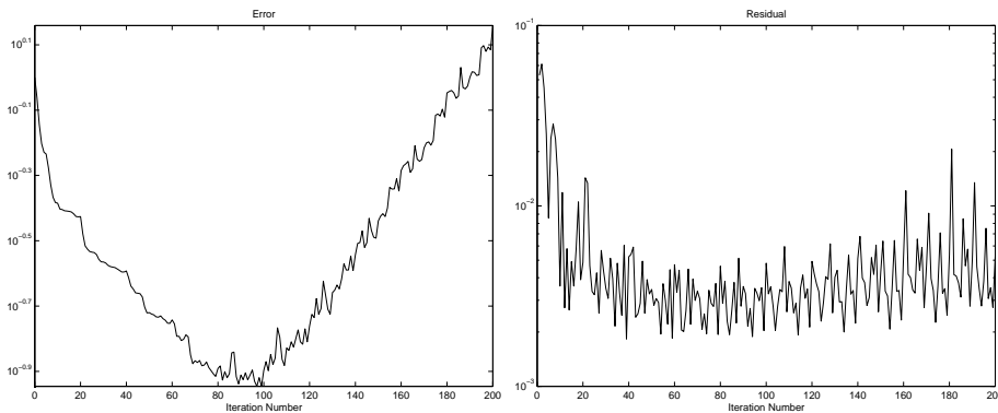
FIG. 5.9. Semi-logarithmic plot of error (left) and residual (right) vs. iteration number in the second example, \delta = 0.5\%
