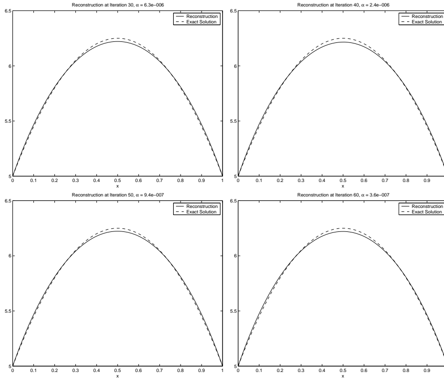
FIG. 5.2. Reconstructions in the first example, \delta = 0 , at iterates 30, 40, 50, and 60
