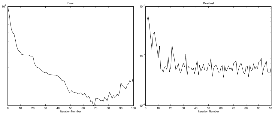
FIG. 5.8. Semi-logarithmic plot of error (left) and residual (right) vs. iteration number in the second example, \delta = 1\%
