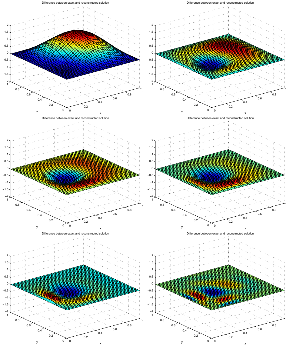
FIG. 5.6. Difference \hat{q} - q_n in the second example at iterates 1, 2, 3, 5, 10, and 100.
