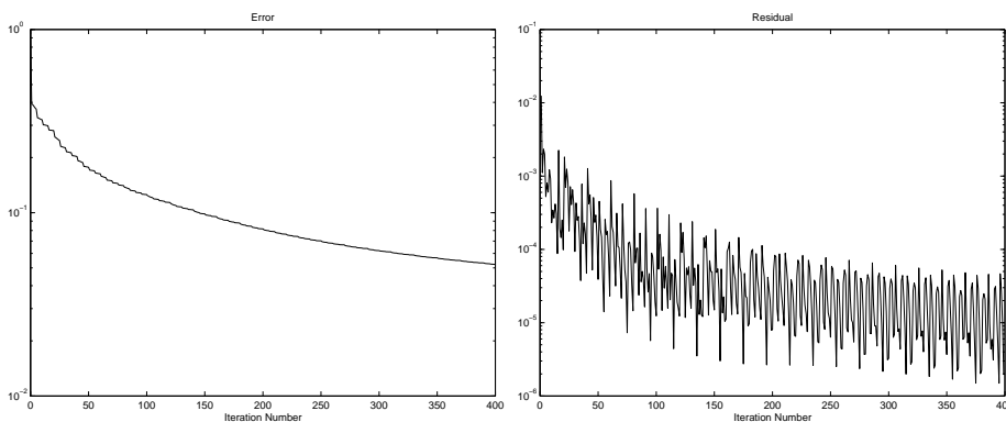
FIG. 5.10. Semi-logarithmic plot of error (left) and residual (right) vs. iteration number in the second example for different exact solution, \delta = 0
