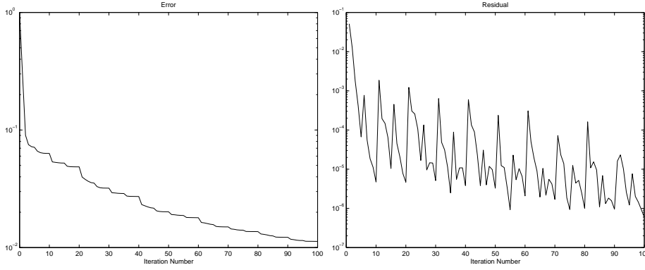
FIG. 5.7. Semi-logarithmic plot of error (left) and residual (right) vs. iteration number in the second example, \delta = 0
