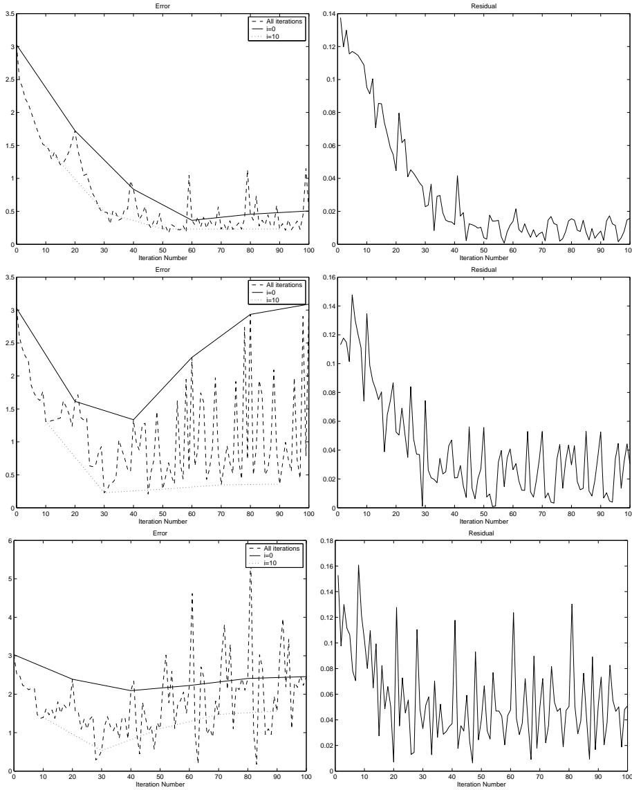
FIG. 5.5. Plot of error (left) and residual (right) vs. iteration number in the first example, for noise levels \delta = 1\% (top), \delta = 3\% (middle), \delta = 5\% (bottom)
