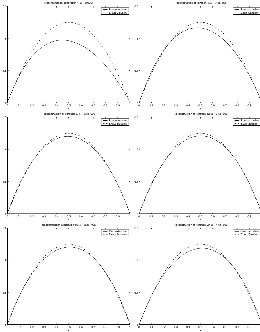
FIG. 5.1. Reconstructions in the first example, \delta = 0 , at iterates 1, 4, 8, 12, 16, and 20
