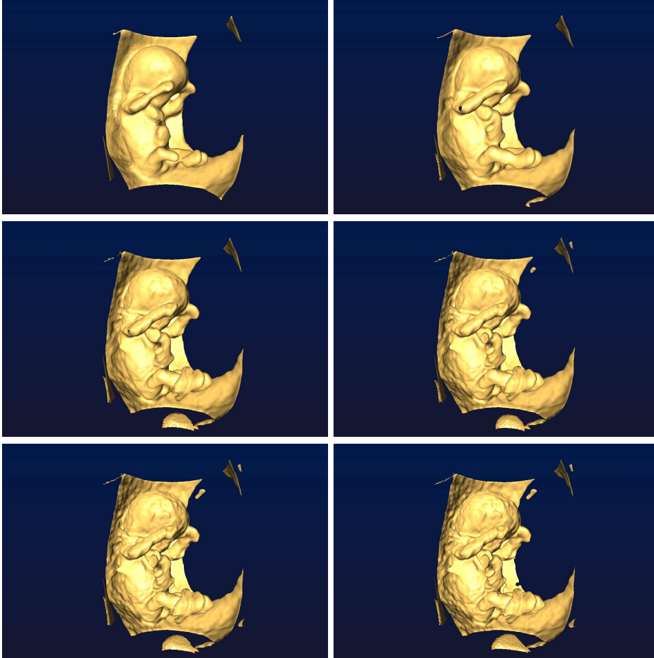
FIGURE 3. Denoised surfaces: Steps 1, . . . , 6 with \alpha = 0.5 .
