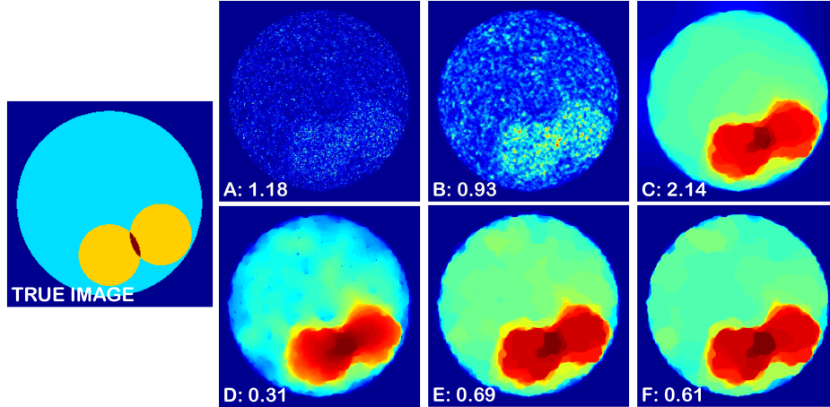
Fig. 1. Synthetic object: results of different reconstruction methods and Kullback-Leibler distances to true image. A: EM reconstruction, 18 its. B: EM, 18 its, with Gaussian smoothing any 5th step. C: A with standard ROF smoothing, (1) with (2). D: A with weighted ROF smoothing (10). E: A with iterative weighted ROF smoothing (9), 30 its. F: Nested EM-TV algorithm (6), 30 its.
