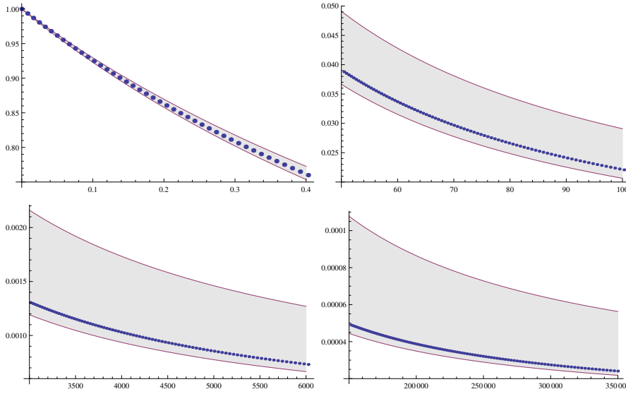
Fig. 2 Comparison between the numerical solution b \mapsto G_{0b} (obtained in [17]) of the equation (4) for \lambda = -\frac{1}{2\pi} (blue dots) with the domain \exp(\mathcal{K}_\lambda) (shaded region, defined in (7)) in which we proved existence of a fixed point. Observe the big variation of b -intervals and corresponding values G_{0b} .
