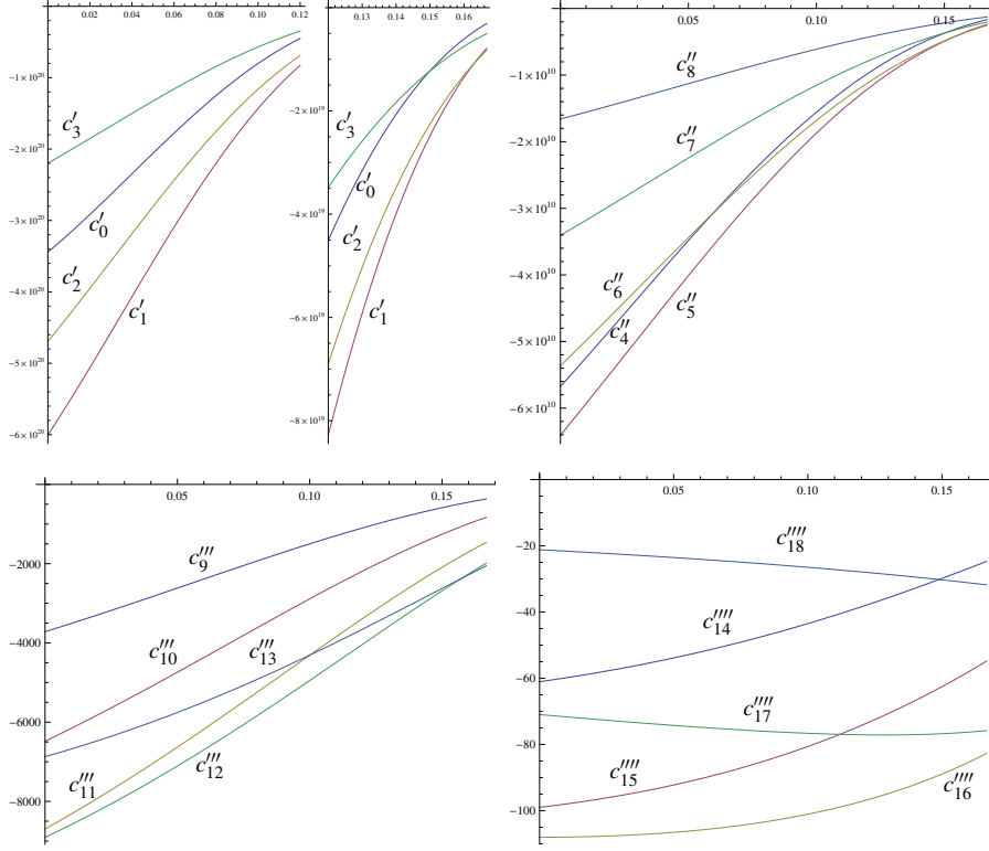
Fig. 1 Plot of the rescaled coefficients c'_k(\lambda) := (20\lambda)^{17-k} c_k , c''_k(\lambda) := (4\lambda)^{17-k} c_k , c'''_k(\lambda) := (\frac{2}{6})^{17-k} c_k and c''''_k(\lambda) := (\frac{2\lambda}{3})^{17-k} c_k . All of them are manifestly negative.
